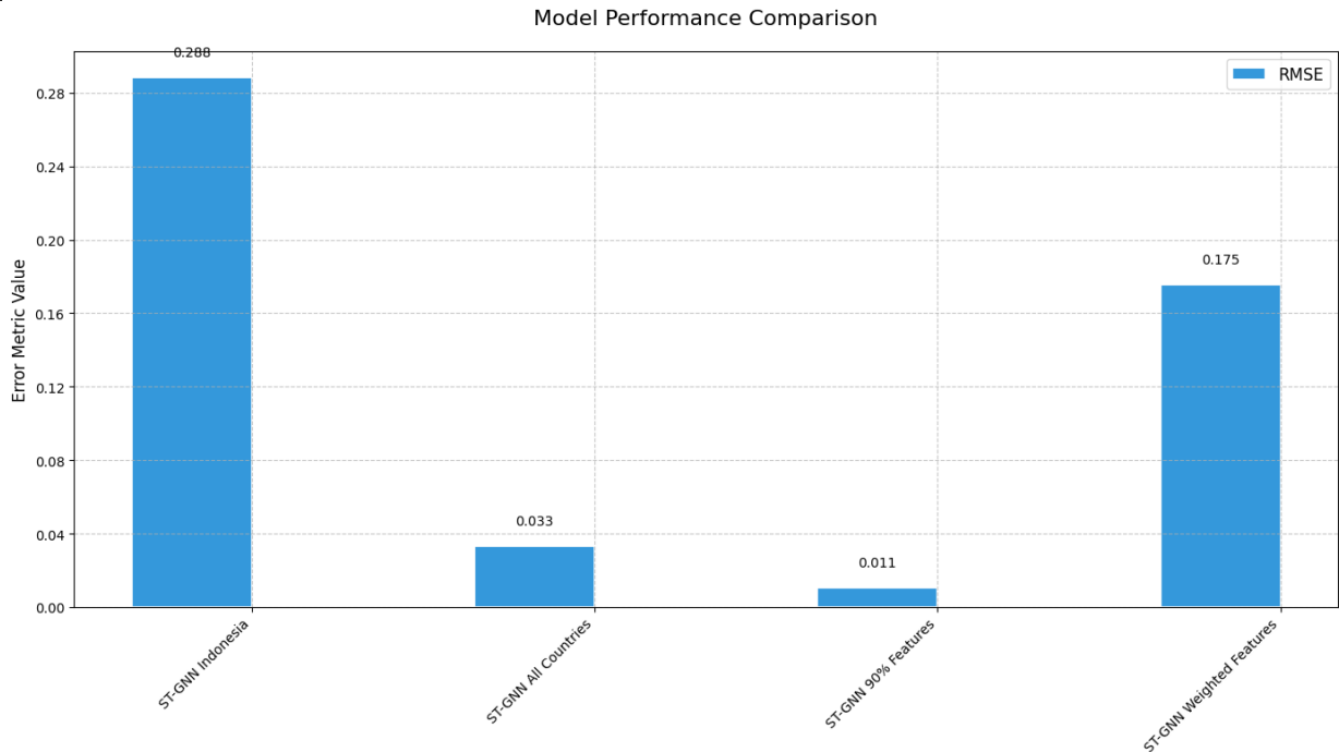
Figure 7. Model Performance
